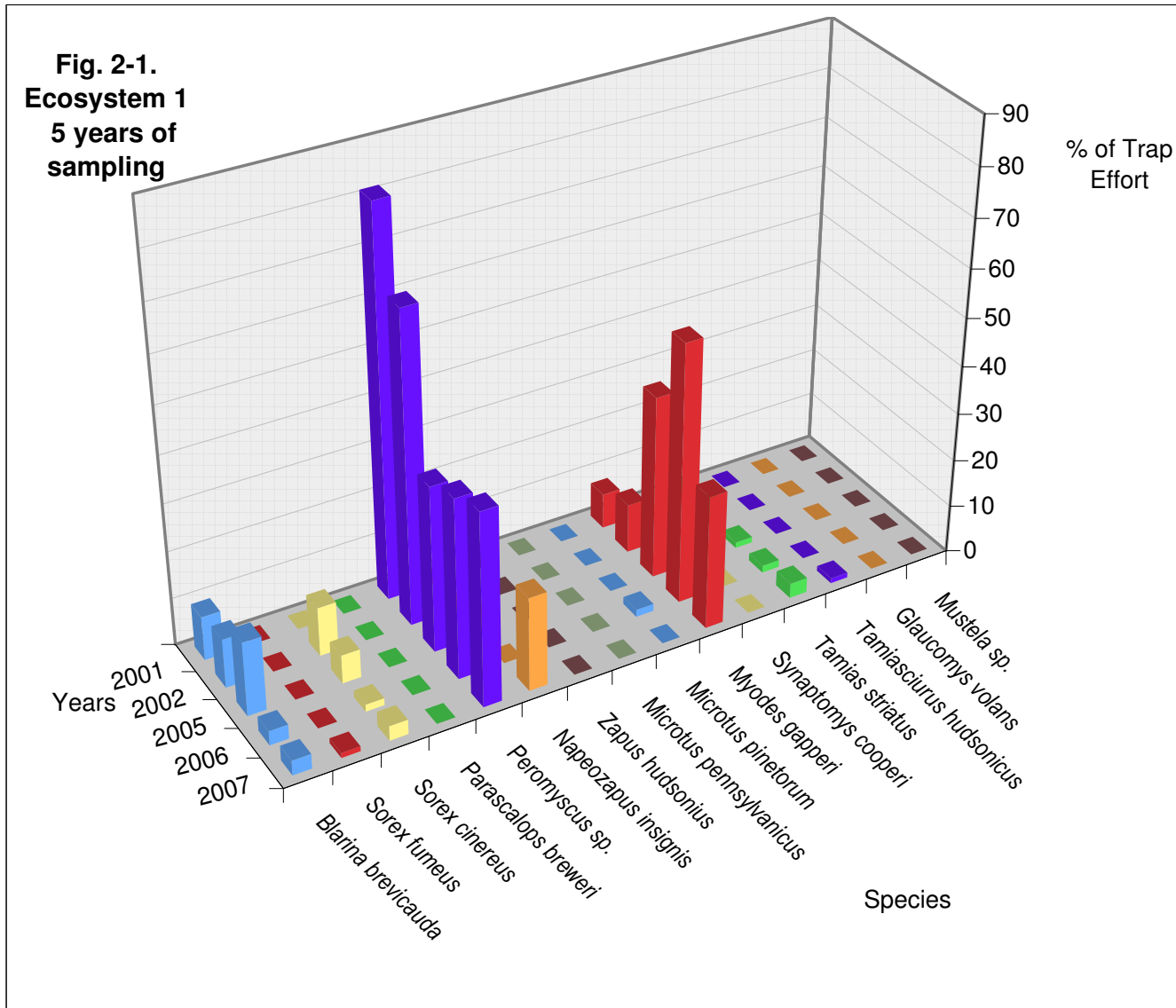
Figure 2. 3-D graphs of 5 and 6-year species frequencies in the four ecosystems monitored on Guthrie-Bancroft expressed as percent of trap effort (compare data in Table 1.2).
